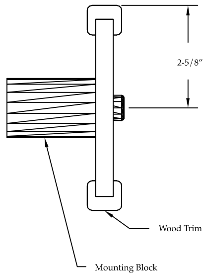
Bellagard Chair Rail w/ wood top and bottom caps
