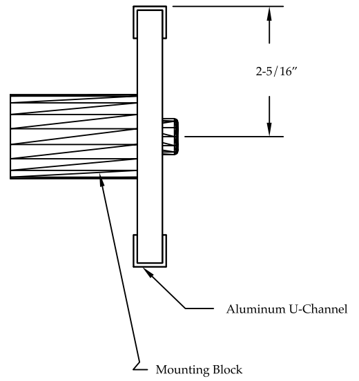
Bellagard Chair Rail w/ aluminum top and bottom caps
